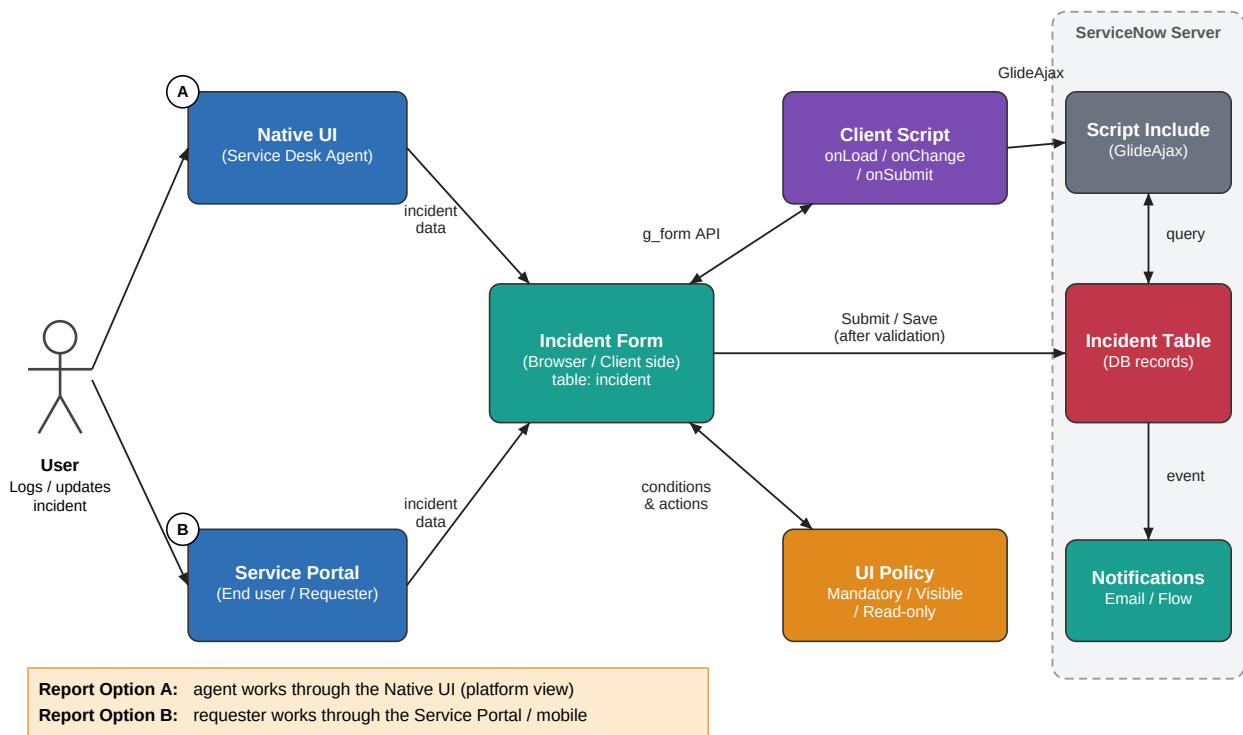
Figure 1: Architecture and data flow of the Incident form with Client Script and UI Policy in ServiceNow
